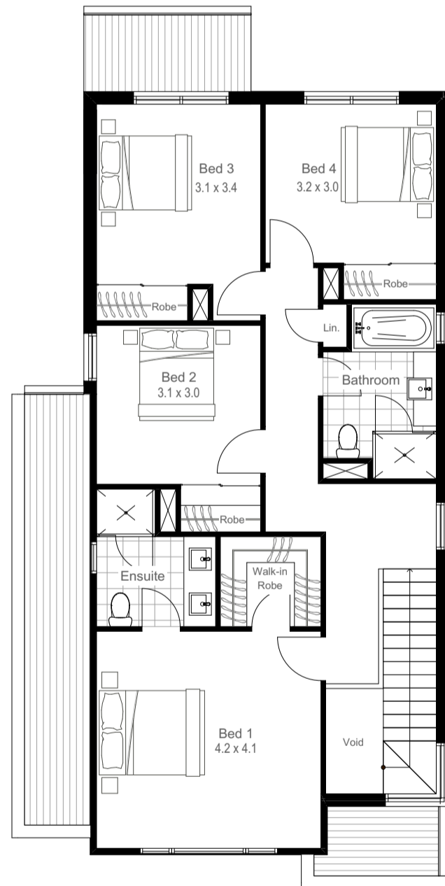
UPPER FLOOR
